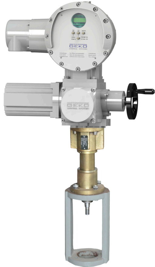
Explosion-proof type
